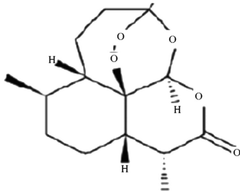
Figure 2. Artemisinin.
