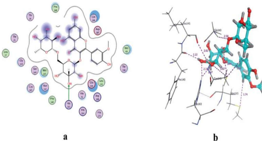
Fig. 2. (a) 2D and (b) 3D representation of docking of flavonoid into the N3 binding site of the COVID-19 Mpro (44).
