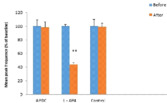
Fig. 5. Effect of drugs on Mean peak frequency of SWDs. Reduction of mean Peak frequency before and after drug injection by paired t-test indicate that only L-AP4 was significant. L-AP4 reduce mean peak frequency more than other groups. Values are mean \pm SE, ** p < 0.01 .
