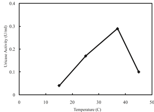
Fig. 6. Thermal stability of crude uricase
