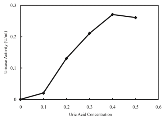
Fig. 8. The effect of uric acid concentration on uricase activity
