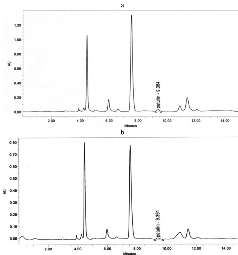
Figure 2. (a) Chromatogram for apple juice spiked with 50 µg L -1 of patulin, and (b) Chromatogram for a contaminated apple juice.
