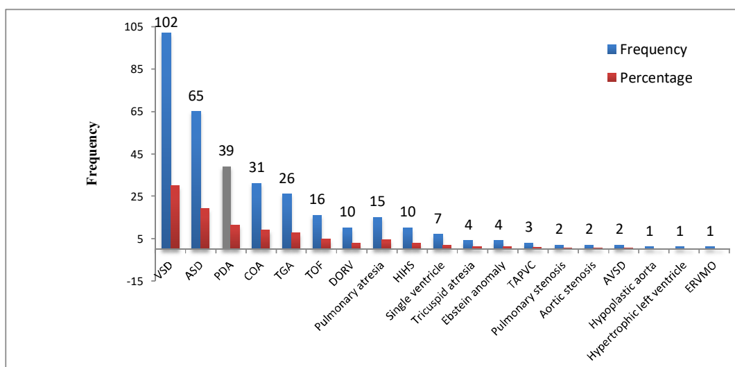
Fig. 1. Frequency of different types of CHD
